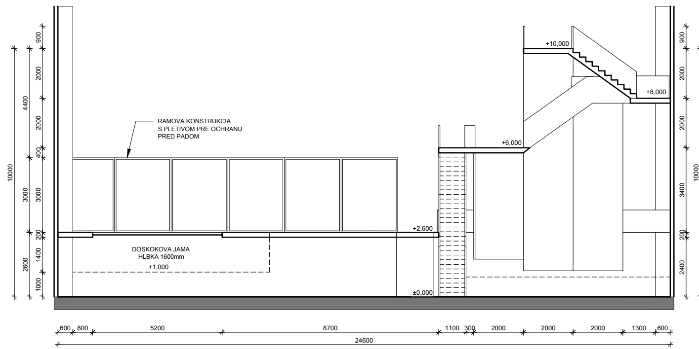
Rez C
