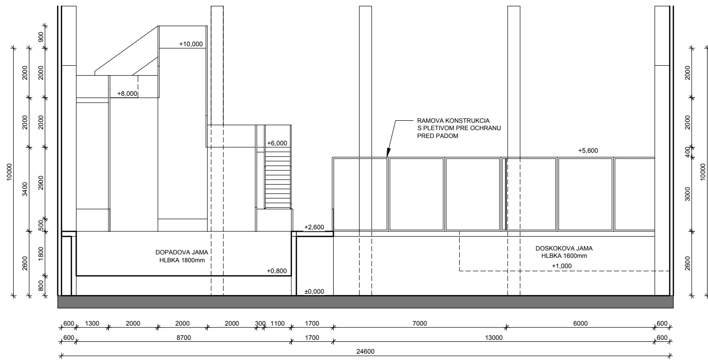
Rez A
